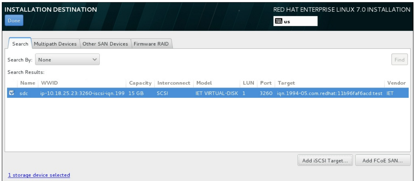
Figure 13.30. Tabbed Overview of Specialized Storage Devices
