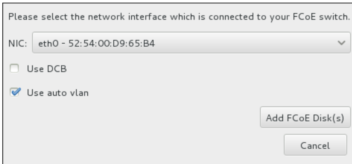
Figure 13.35. Configure FCoE Parameters
