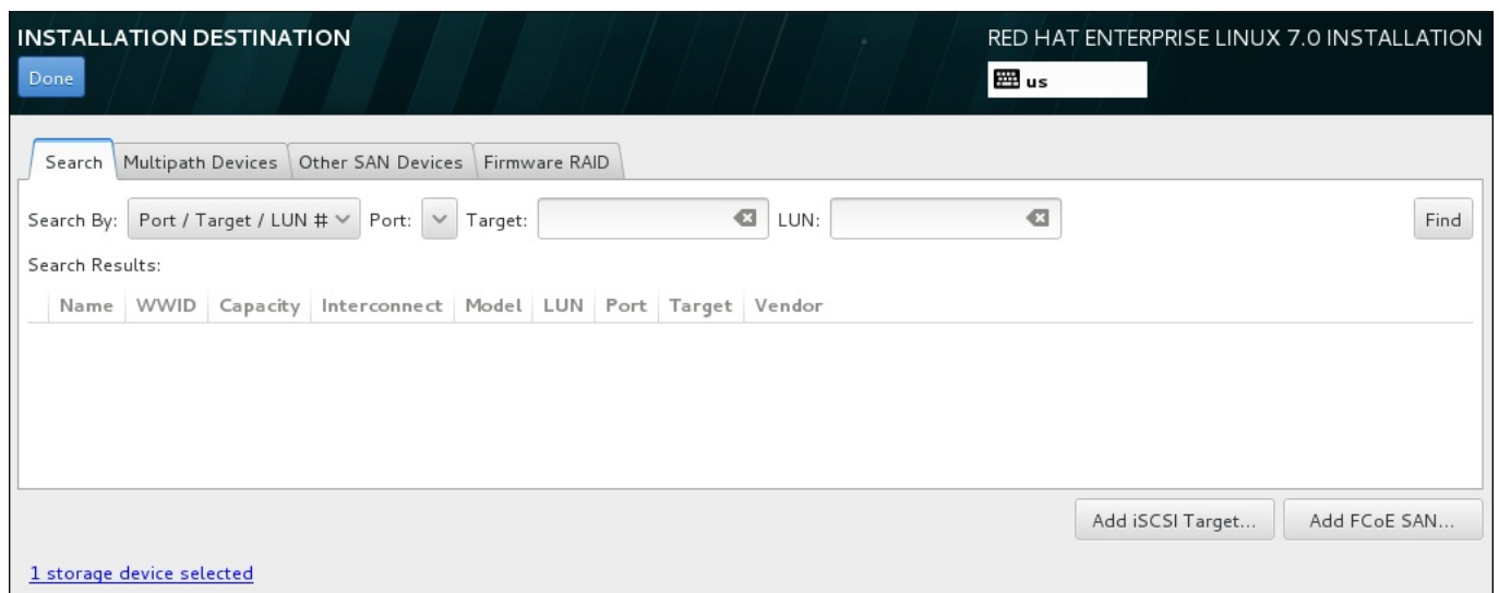
Figure 8.32. Advanced Storage Options
