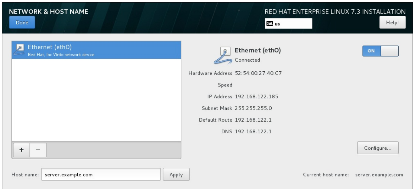
Figure 17.10. Network & Hostname Configuration Screen
