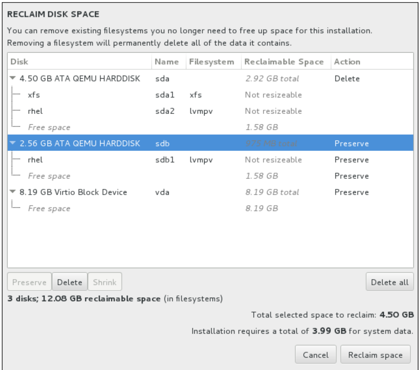
Figure 8.21. Reclaim Disk Space from Existing File Systems
