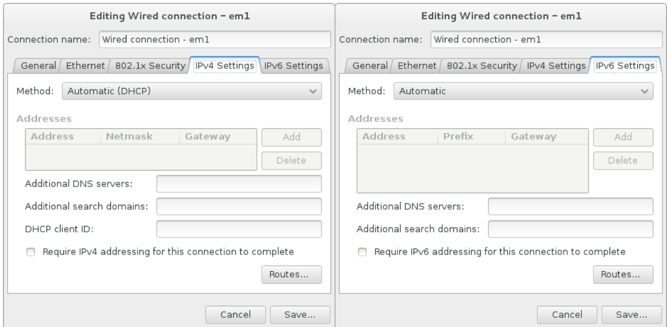
Figure 17.12. IP Protocol Settings
